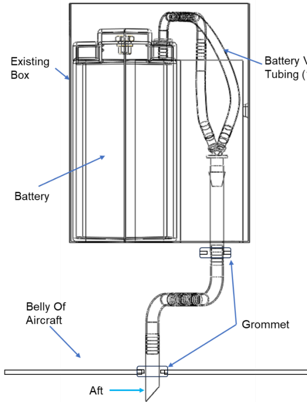
Offset Tube Routing Example
