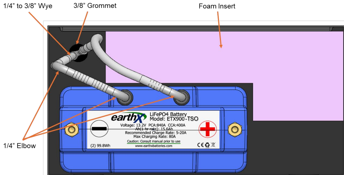
Typical Install for Beechcraft, Navion
