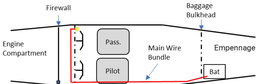
Piper/Mooney/Beechcraft/Ercoeur/Luscombe/Rockwell/Navion/Bellanca Wire Routing
