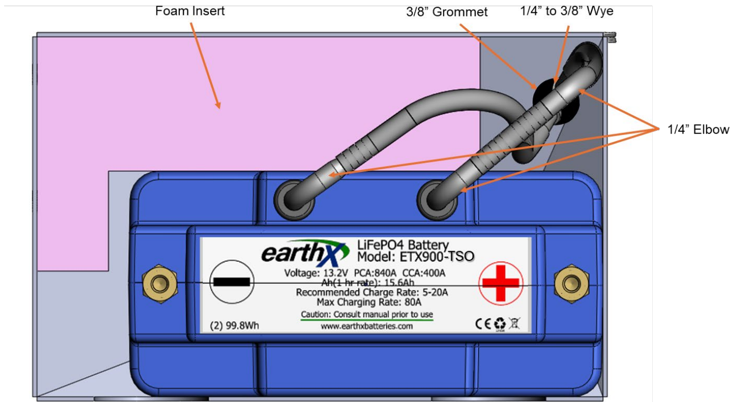
Typical Install for C150, 170,172
