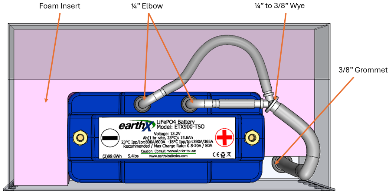
Typical Install for Commander, Stinson, Cessna 190, Cessna 195, Cessna 206
