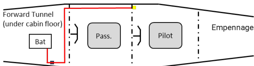
Game Bird GB1, Extra EA 300/200, Extra NG Wire Routing
