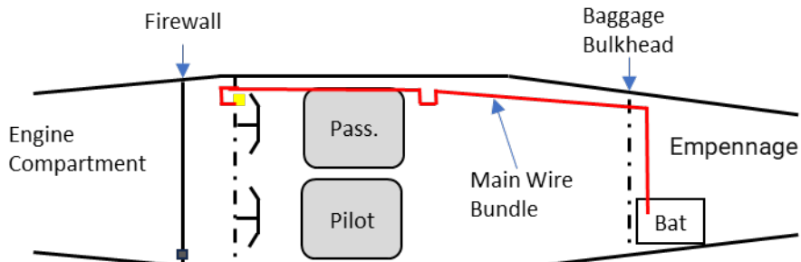
Cessna 120/140/150/170/172/177/180/182/185/190/195 Wire Routing
