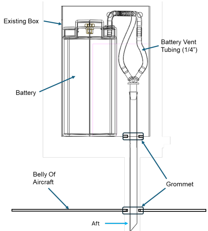
Straight Tube Routing Example
