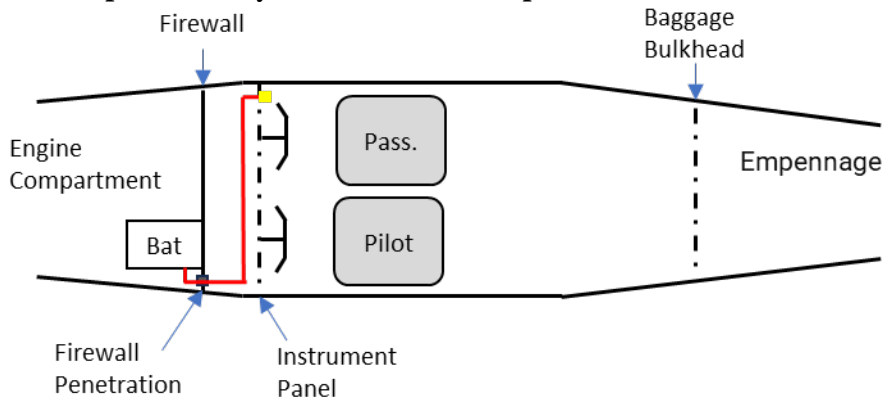
Cessna 150/170/172/206/210 Wire Routing
