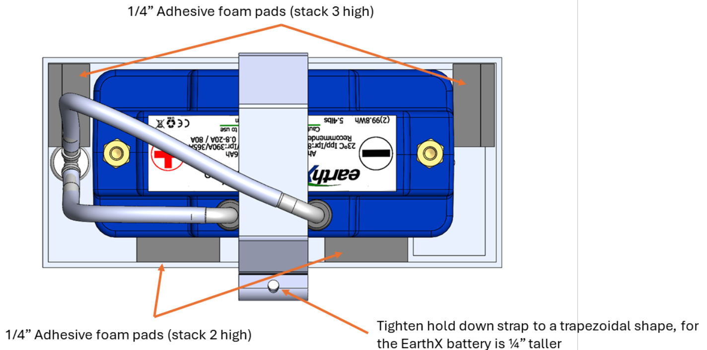
Typical Firewall Installation
