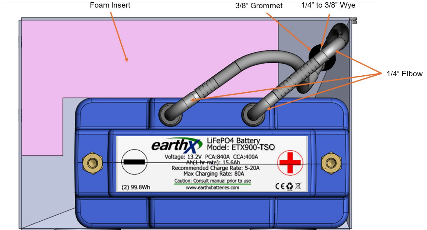
Typical Install
