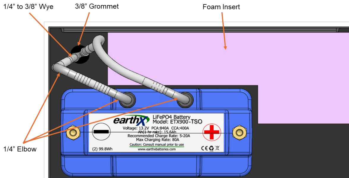
Typical Install for Beechcraft 19 23 25, Navion, Swift
