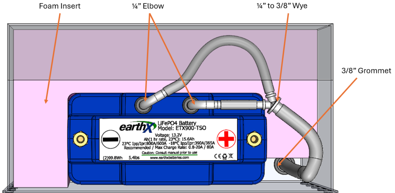
Typical Install for Commander, Stinson, Cessna 190, Cessna 195, Cessna 206, Beechcraft Bonanza
